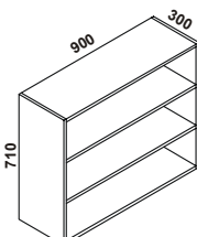
H90 - korpus police
