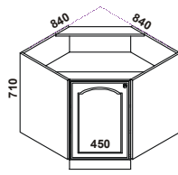
SRS45 + P45/71 + K4
