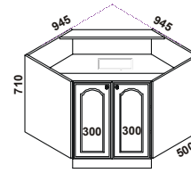
SRS60 + 2xP30/71 + 2xK4
