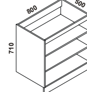
S80 - korpus police
